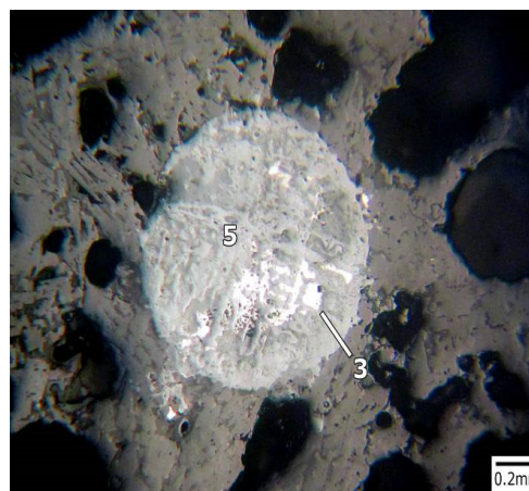
Fig.13. Microscopic View of the Slag in Fig.9—a Relatively Large Iron Prill (3) Most Parts of which Were Replaced by Secondary Iron Oxides (5).
