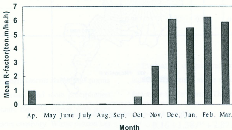
Figure 4 Monthly variation of rainfall erosivity in study area
