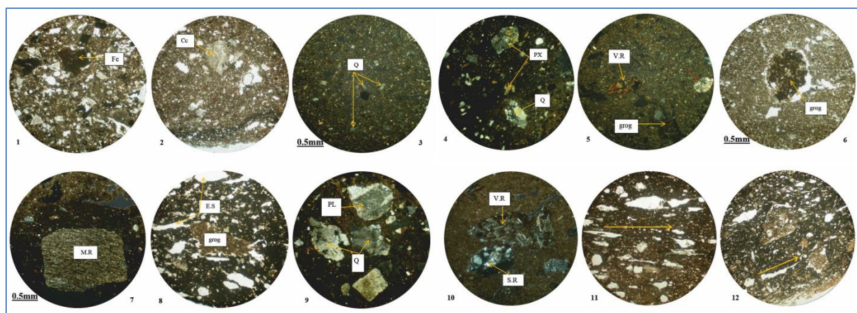
Fig. 4. Photomicrograph, 1 (Tepe Ghabristān. Light PPL, Fe-oxide, light minerals are quartz that seen in micro crystal form at center of picture is calcite in grey color), 2 (Tepe Khāki. Light PPL, residue of burned calcite), 3 (Tepe Vizheh. Light XPL, Silty Texture, quartz in phenocryst and polycrystalline form), 4 (Tepe Ali Baeig. Light XPL, Pyroxene and quartz), 5 (Kalgāh Zamān. Light XPL, volcanic rocks in center, grog are seen in dark), 6 (Tepe Khāki. Light PPL, silt mineral (Grog) is in dark at center, background is combination of silt and tiny carbonates), 7 (Tepe Khāki. Light XPL, metamorphic rock at center), 8 (Kalgāh Zamān. Light PPL, grog and volcanic rock at center and empty space are in light and dark color), 9 (Tepe Āgāh. Light XPL, Polycrystalline quartz and plagioclase), 10 (Tepe Āgāh. Light XPL, sedimentary rock, calcite and volcanic rock.), 11 (Tepe Ali Baeig. Light PPL, visible components and empty space), 12 (Tepe Khāki. Light PPL, visible components and empty space).
