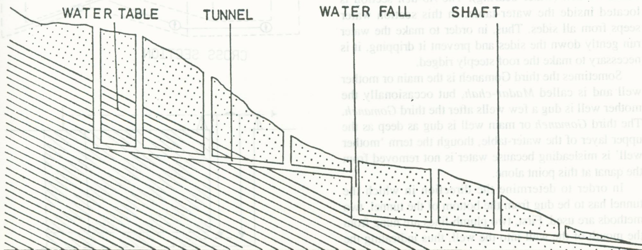
Fig.4 WATERFALL IN QANAT SYSTEM
