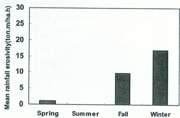
Figure 5 Seasonal variation of rainfall erosivity
